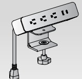
PM5311B Black PM5311W White Power Charger Clamp-Mount Includes: USB Type-C, USB Type-A & (3) A/C plugs Fits 1/2"-1 1/2" surfaces $275
